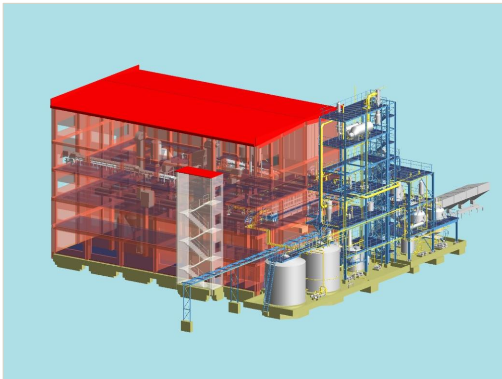
FIG. 05 – IPE MODEL: PDMS model of the revamped unit by IPE, 2007–2008
