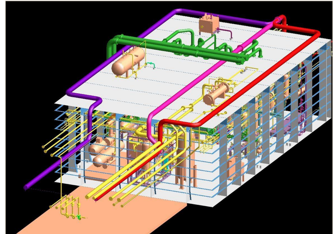
FIG. 08 – IPE MODEL: compressor-house module of the Multigas LNG/LPG carrier in PDMS, 2008
