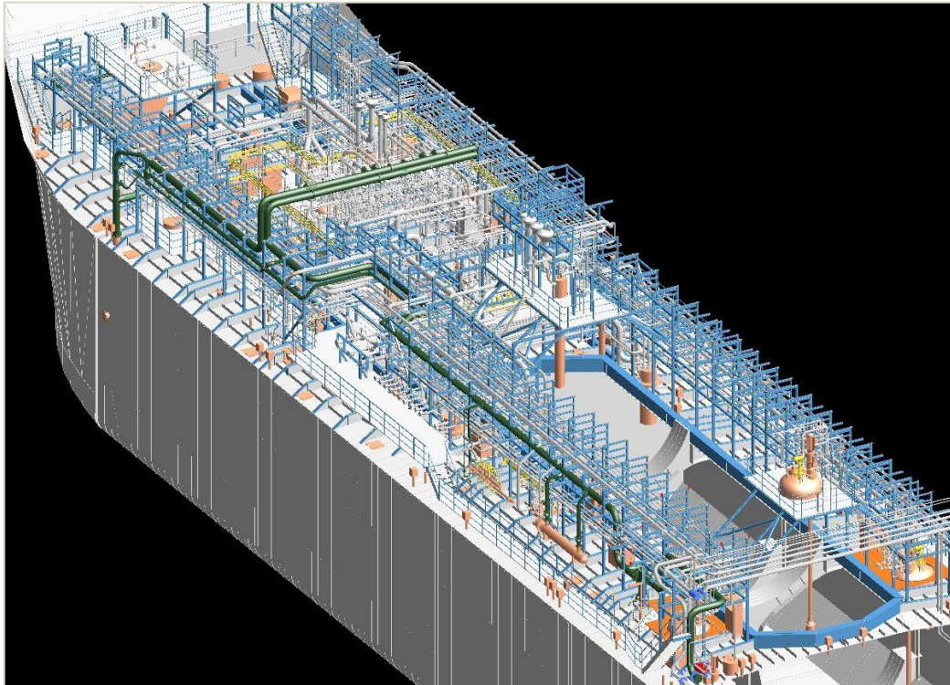
FIG. 07 – IPE MODEL: deck of the Wintergas LPG carrier in PDMS, seawater-cooling system highlighted, 2007
