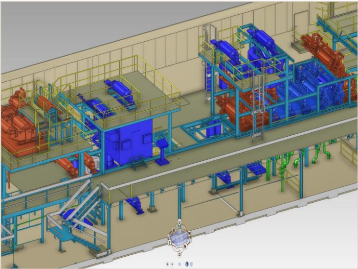
FIG. 03 — Tinning line EC1 with the new passivation equipment · IPE 3D model, 2021–2024
